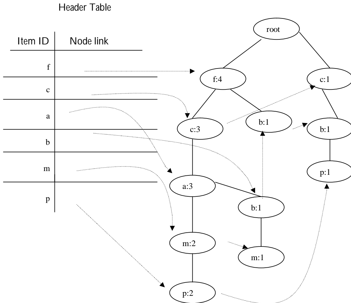
Figure 2: Sample FP-tree for database T
