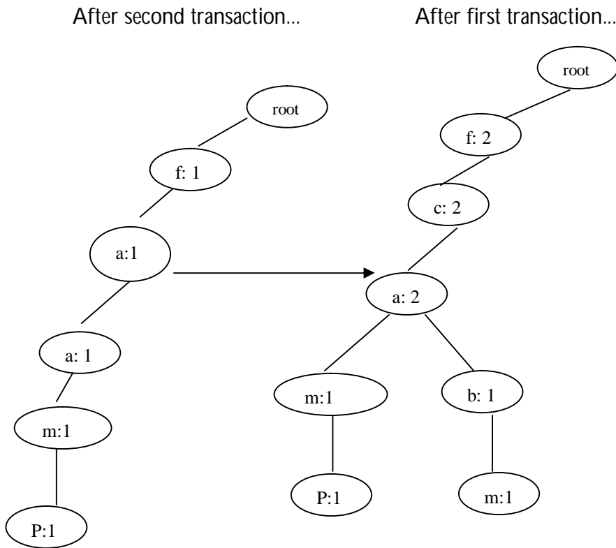
Figure 1: FP-tree after insertion of two transactions
